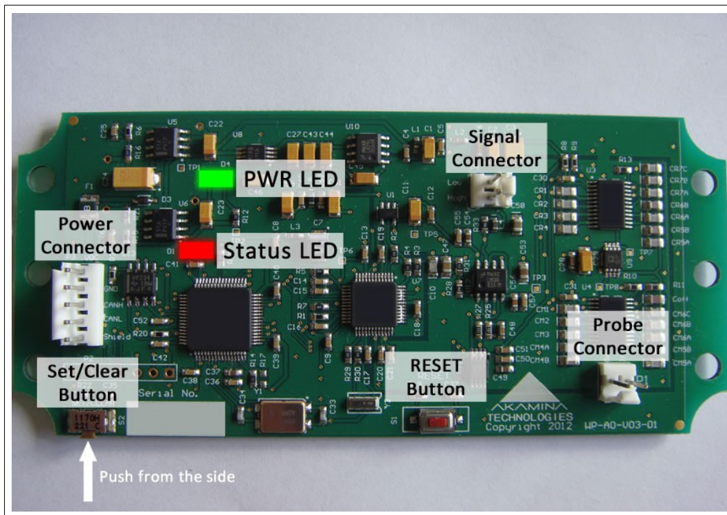
Figure 2-3: AWP-24-2 Circuit Board
