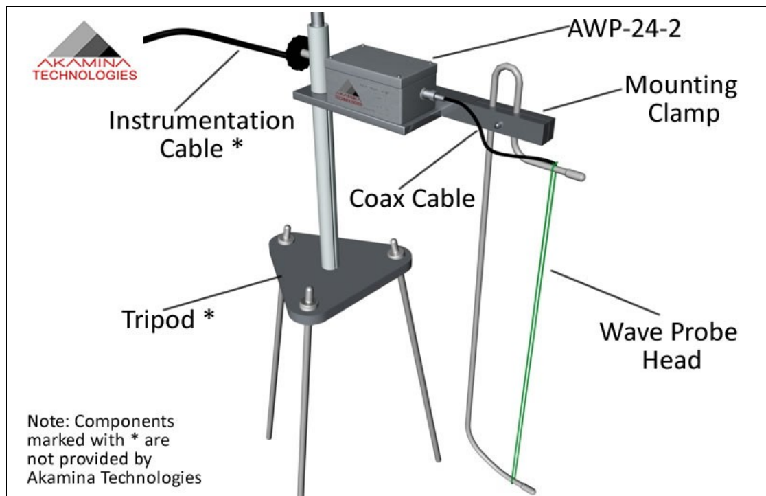
Figure 1-1: AWP-24-2 Wave Height Gauge and tripod
